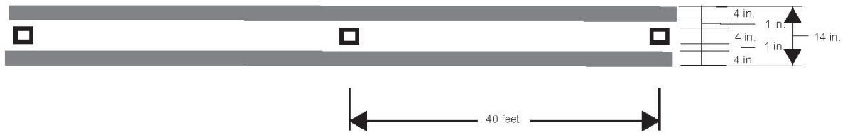
CENTERLINE FOR ALL TWO LANE TWO-WAY ROADWAYS NO PASSING ZONE
