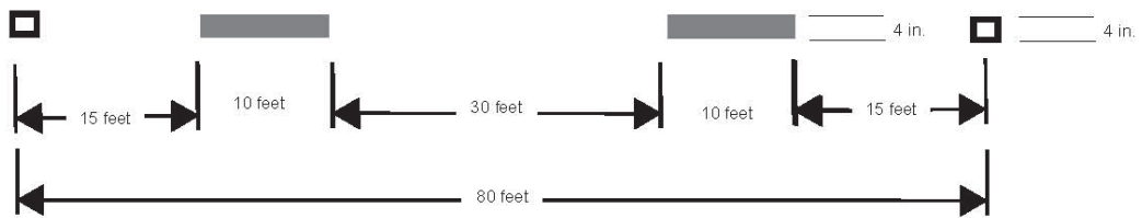
CENTERLINE FOR ALL TWO LANE TWO-WAY ROADWAYS REFLECTIVE RAISED PAVEMENT MARKERS GUIDANCE
